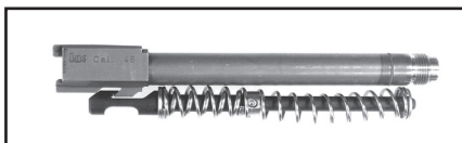
Figure 12 - Proper Position for the Captured Recoil/Buffer Spring Assembly on the Barrel Locking Block
