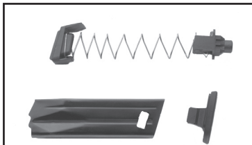
Figure 11B 10-Round Magazine (Disassembled)
