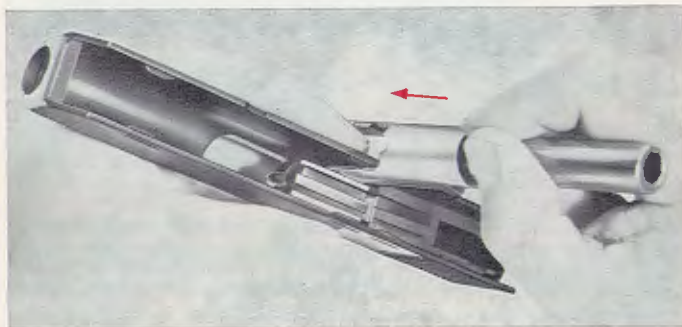
Fig. 11: Press against the locking lever
